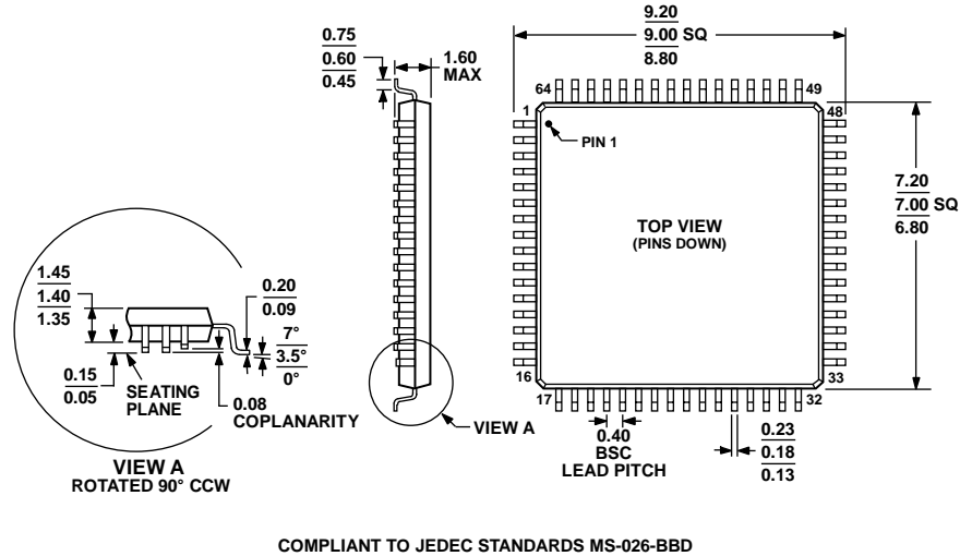
Figure 60. 64-Lead Low Profile Quad Flat Package [LQFP] (ST-64-1)
